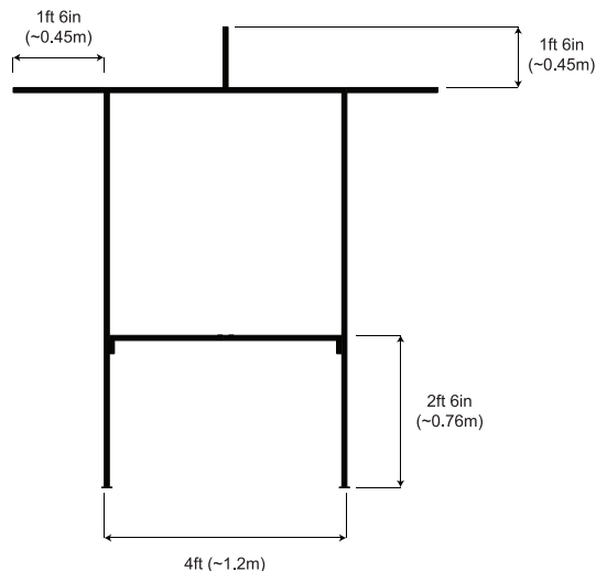
ASSEMBLY
