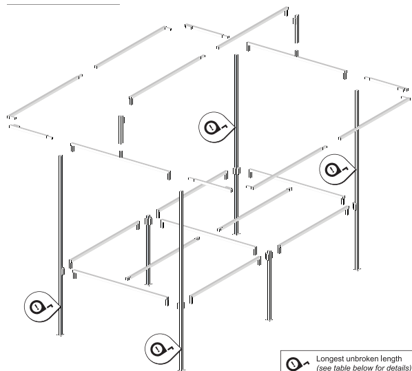
ASSEMBLY
